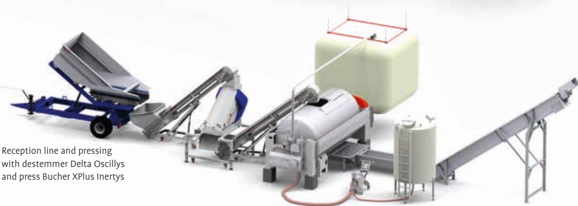
Reception line and pressing with air knife sorting table Delta Rflow and press Bucher XPlus
